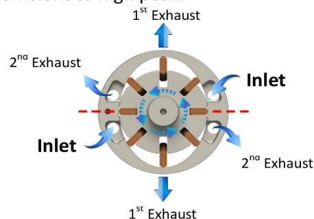
Double Air Intake
