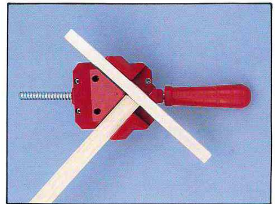
MAKES 90° "L" AND "T" JOINTINGS W/MATERIAL OF DIFFERENT THICKNESS
