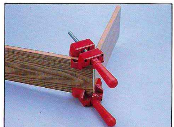
ACCURATE RECTANGULAR HOLDING FOR WOOD PLATES
